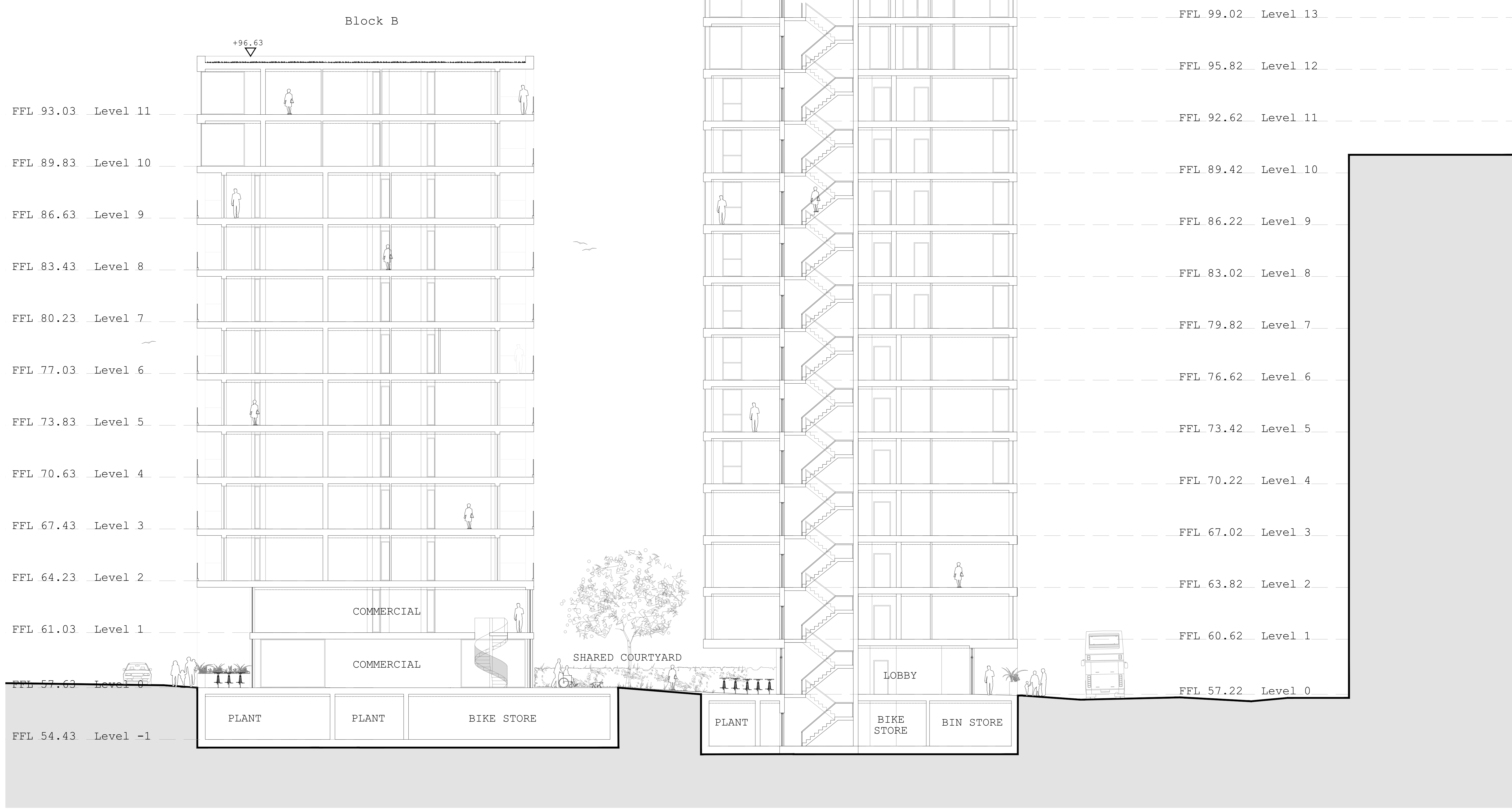
PROPOSED SECTION 2-2'
