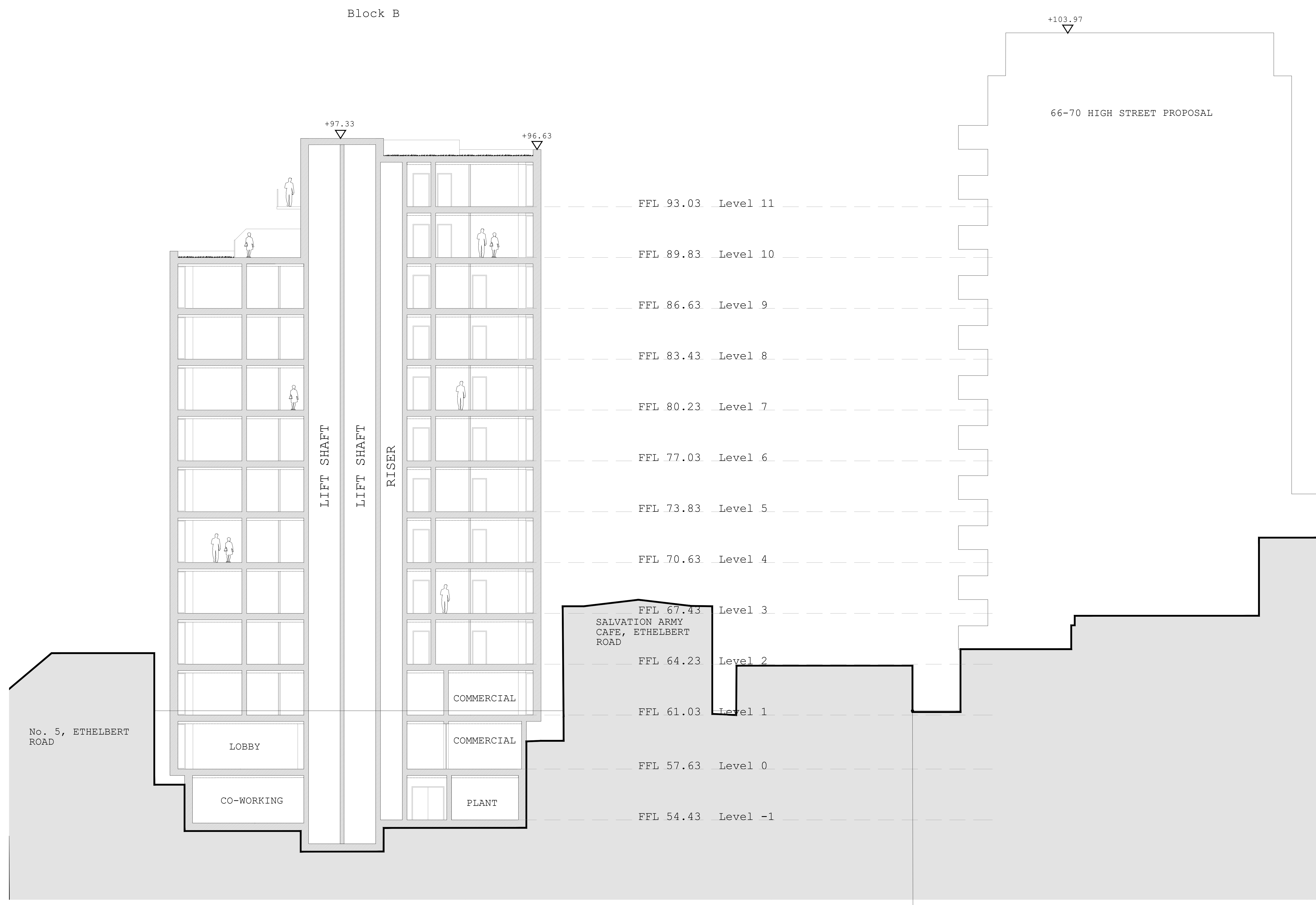
PROPOSED SECTION A-A' 1:1008A0 0 1 2 3 4 5M
