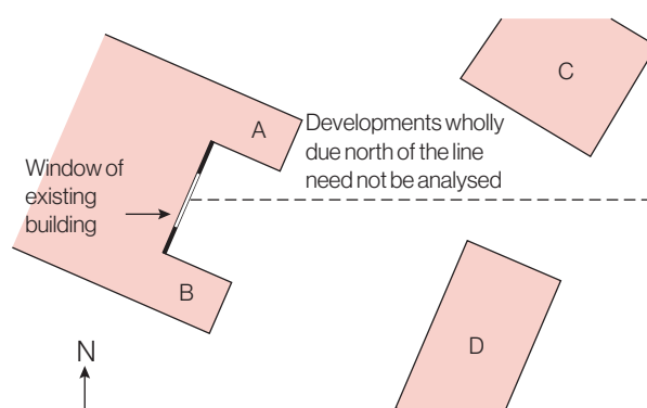
Figure 27: In analysing the sunlighting impact on the existing window, no check need be made for proposed extension A and new building C, as they lie within 90^\circ of due north of the window. Proposed extension B should be checked, as should new building D if it subtends more than 25^\circ to the horizontal, measured in section from the centre of the window
