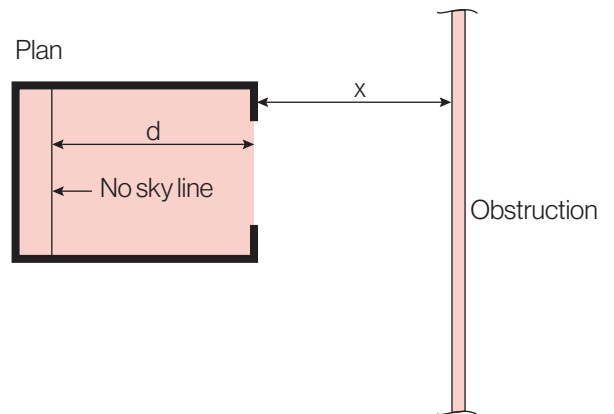
Figure D3: For a long horizontal obstruction parallel to the window, the no sky line is also parallel to the window. Its position can be found from the section.
