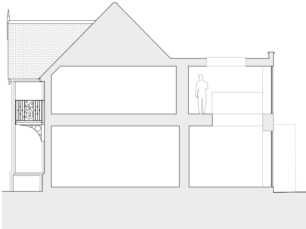
GREENACRES - Section A & Elevation 1:100 @ A1
