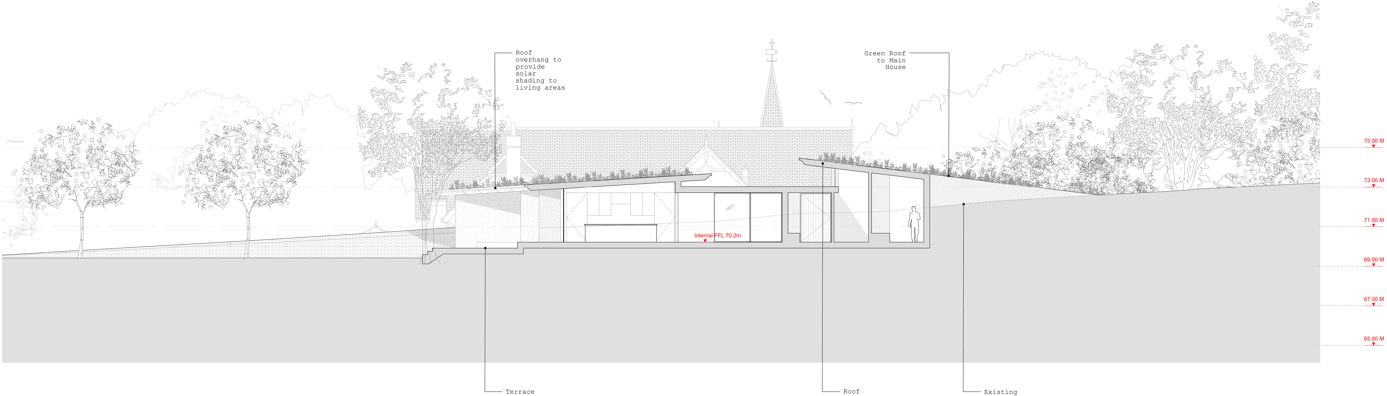
Section B 1:100 @ A1
